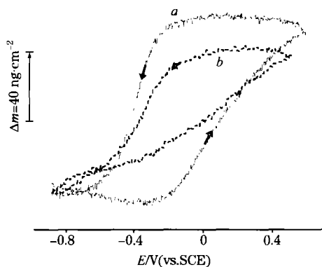
Fig 3 \Delta m variation of Pt electrode in 0.1 \text{ mol} \cdot \text{L}^{-1} t butanol and 0.1 \text{ mol} \cdot \text{L}^{-1} NaOH solution; sweep rate 50 \text{ mV} \cdot \text{s}^{-1}
