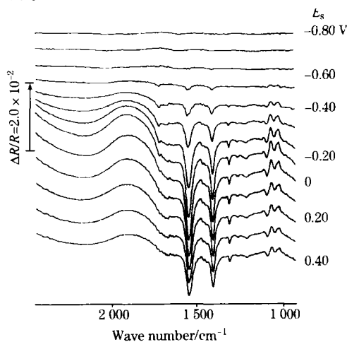
Fig 2 Difference spectra obtained with a Pt electrode in 0.1 \text{ mol} \cdot \text{L}^{-1} t-butanol + 0.1 \text{ mol} \cdot \text{L}^{-1} \text{ NaOH} solution. The reference potential E_R was at -0.90 \text{ V} and the value of potential E_S for each spectrum is indicated in the figure
