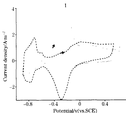
Fig 1 Cyclic voltammogram of Pt electrode in 0.1 \text{ mol} \cdot \text{L}^{-1} t-butanol and 0.1 \text{ mol} \cdot \text{L}^{-1} \text{ NaOH} solution
