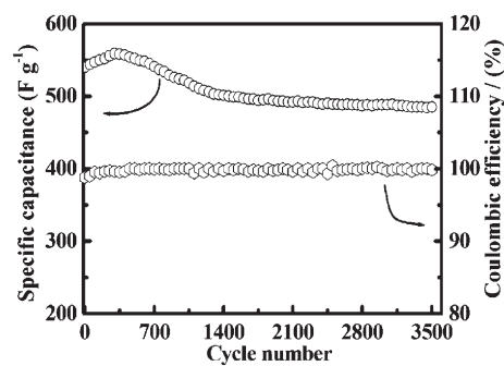
Fig. 8 Cycling performance and coulombic efficiency of the mesoporous hollow NiCo 2 O 4 sub-microsphere electrode as a function of cycle number at 10 A g -1 .
