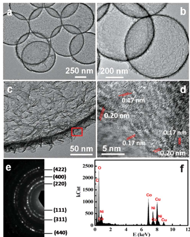
Fig. 3 (a–c) TEM and (d) HRTEM images, (e) SAED pattern and (f) EDAX of the hollow \text{NiCo}_2\text{O}_4 sub-microspheres. The image in (d) is taken from the region marked with the rectangle in panel c.
