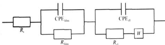
图7 MCMB/Li 电池等效电路 Fig.7 Equivalent circuit for MCMB/Li cell
