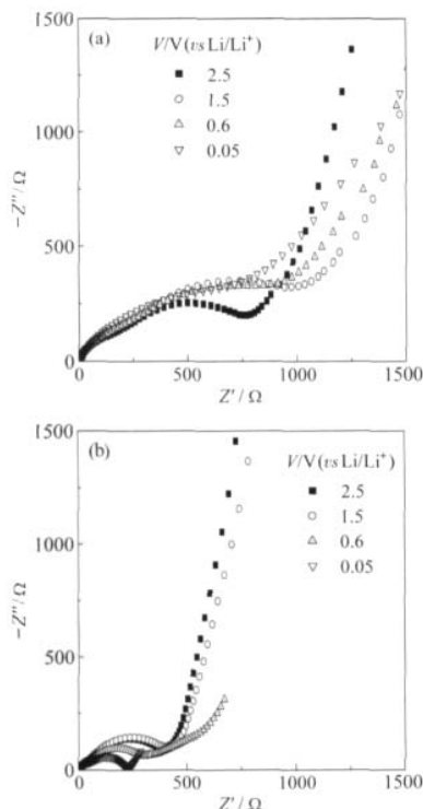
图6 MCMB/Li电池首次放电至不同电压时的Nyquist图 Fig.6 Nyquist plots for MCMB/Li cell measured at different voltages (a) without additive; (b) with 2% FEC
