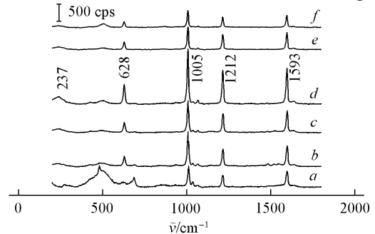
Fig 4 Potential dependent SERS spectra on the Py adsorbed on Au-Co/GC in 0.01 mol/L Py + 0.1 mol/L \text{NaClO}_4 a -0.8 V; b -0.9 V; c -1.0 V; d -1.1 V; e -1.2 V; f -1.3 V.
