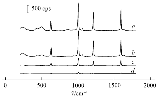
Fig 3 SERS spectra for the Py adsorbed on the Au-Co/GC electrodes at -1.1 V in 0.01 mol/L Py + 0.1 mol/L \text{NaClO}_4 with different Co shell thicknesses a 0.7 nm; b 1.5 nm; c 2.5 nm; d 5 nm.
