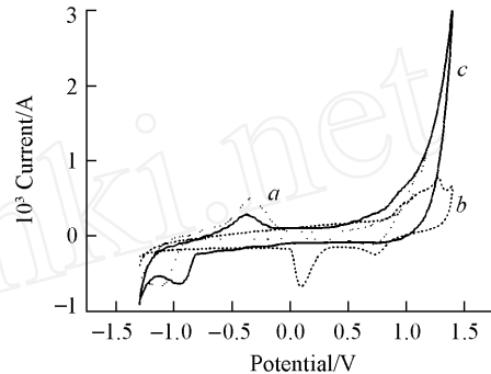
Fig 2 Cyclic voltammograms of Co/GC (a), Au/GC (b) and Au-Co/GC (c) electrodes in 0.5 mol/L \text{NaClO}_4 solution
