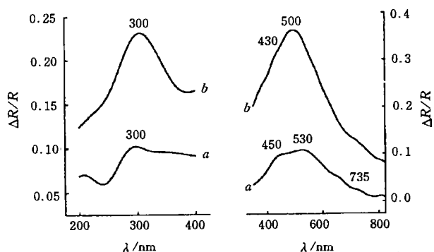
Fig. 3 The in-situ steady state UV-Vis subtractive reflectance spectra of the P- o -PD film electrode in a 1.0 mol/L \text{H}_2\text{SO}_4 solution at potential of 0.04 V/SCE with reference to 0.50 V/SCE (a) and at -0.20 V/SCE with reference to 0.04 V/SCE (b)
