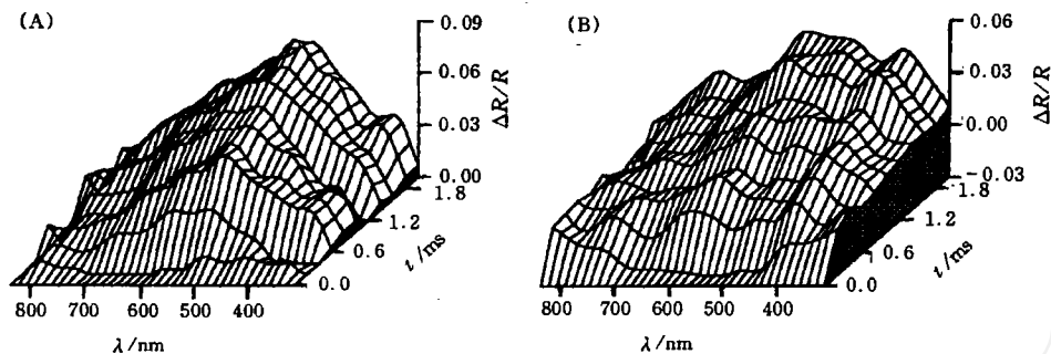
Fig. 4 The in-situ time-resolved UV-Vis subtractive reflectance spectra of the P-o-PD film electrode obtained at potential of 0.04 V/SCE with reference to 0.50 V/SCE(A) and -0.20 V/SCE with reference to 0.04 V/SCE(B)
