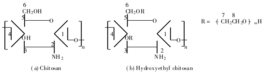
Fig. 1 Chemical structure of chitosan and hydroxyethyl chitosan
