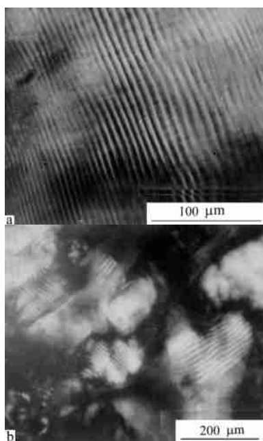
Fig. 4 POM photograph of cholesteric liquid crystal texture of HECS solution a) HECS4 in 30% formic acid solution; b) HECS7 in 18% aqueous solution
