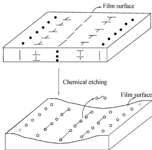
Fig. 5 Model of the mechanism for permanganic etching of HECS cholesteric phase
