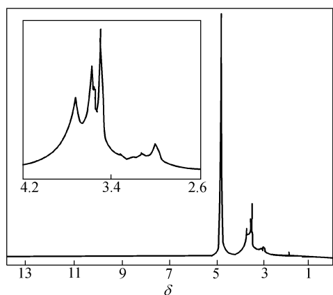
Fig. 3 ^1\text{H-NMR} spectra of HECS2
