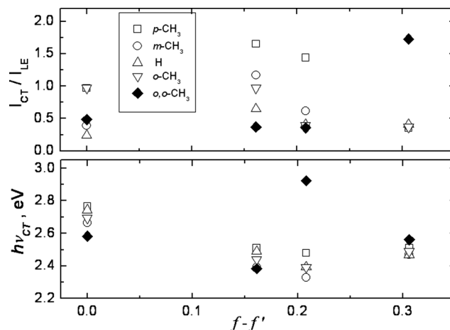
Fig. 4 Variations of the CT to LE emission intensity ratio (up) and CT emission energy (bottom) of DMBA derivatives with different substitutions at the amido aniline moiety in CHX, cyclohexane; DEE, diethyl ether; THF, tetrahydrofuran; and ACN, acetonitrile.
