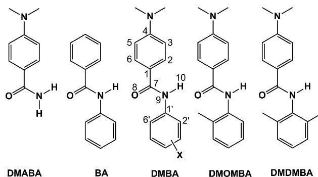
Scheme 1 Molecular structures of investigated compounds. X in DMBA are H, p -CH 3 and m -CH 3 , respectively. The numbers were used to define the dihedral angle.
