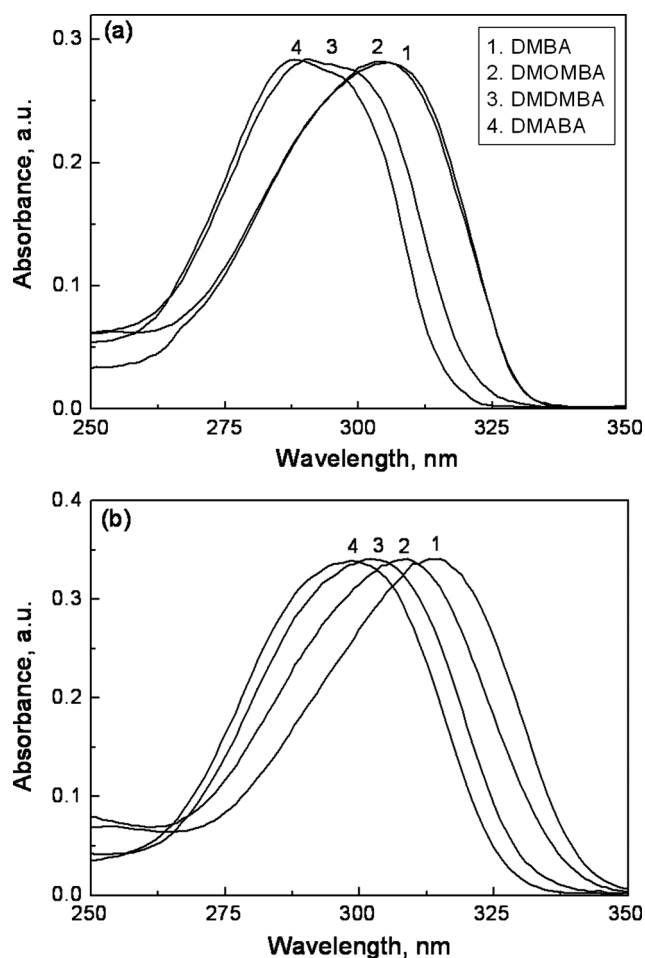
Fig. 1 Normalized absorption spectra of investigated compounds (Scheme 1) in CHX, cyclohexane (a) and ACN, acetonitrile (b).
