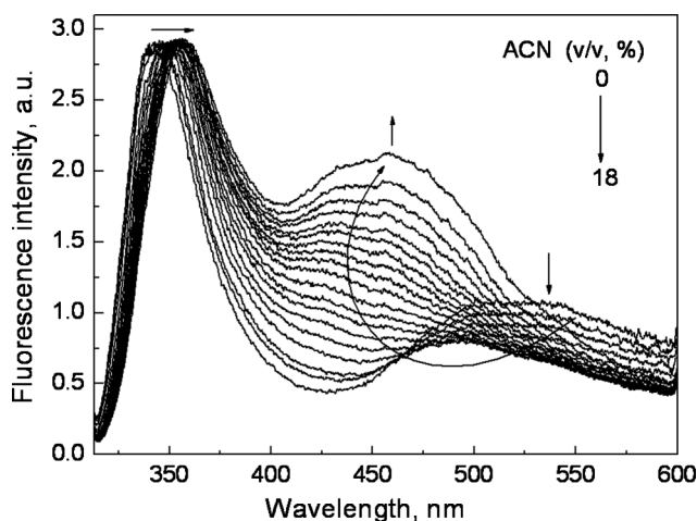
Fig. 3 Fluorescence spectra normalized at LE emission of DMDMBA in DEE with increasing the compositions of ACN from 0 to 18% with interval 1%.
