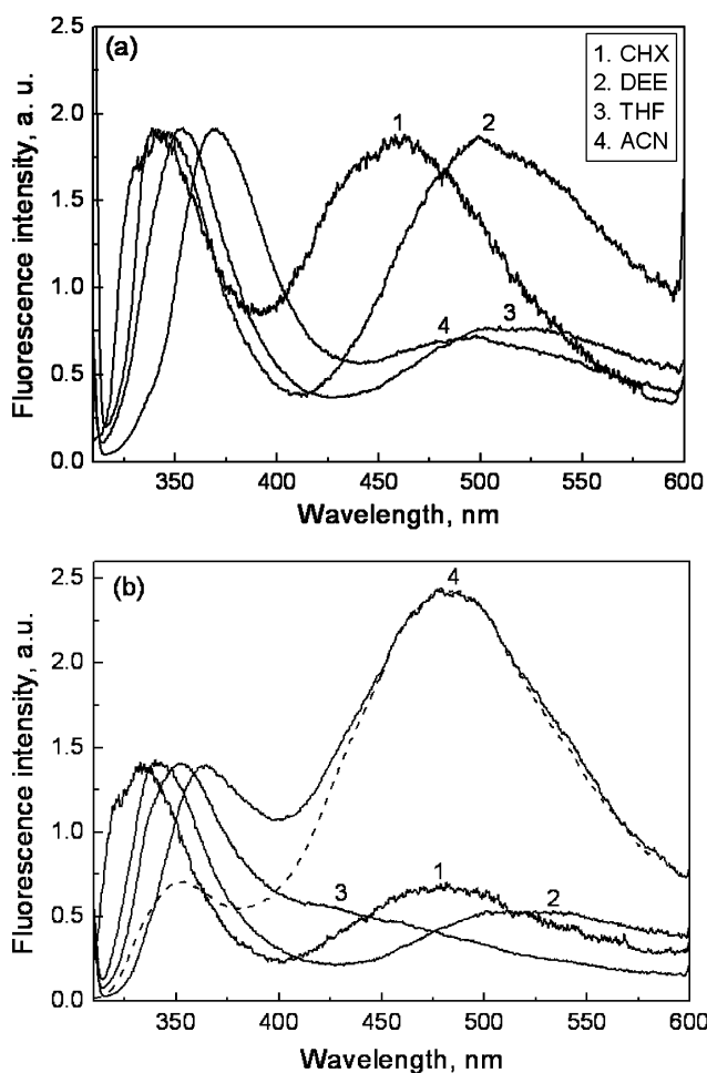
Fig. 2 Fluorescence spectra normalized at LE emission of DMOMBA (a) and DMDMBA (b) in various organic solvents. CHX, cyclohexane; DEE, diethyl ether; THF, tetrahydrofuran; and ACN, acetonitrile. The fluorescence spectra of DMABA in ACN (dashed line) are presented in Fig. 2b for comparison.
