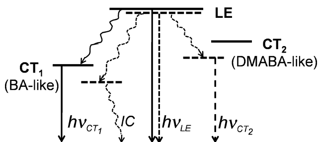
Scheme 2 Illustration of solvent-dependent CT dual fluorescence of DMDMBA in nonpolar solvent CHX (solid line) and polar solvent ACN (dashed line).
