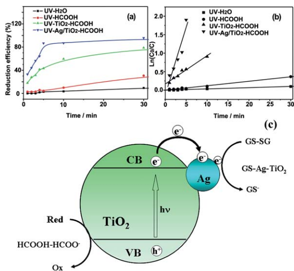
Fig. 2 The reduction efficiencies of GSSG (a), plots of \ln(C_0/C) against t under various reduction systems (b) and possible reduction mechanism of GSSG on Ag/ \text{TiO}_2 nanoparticles (c).
