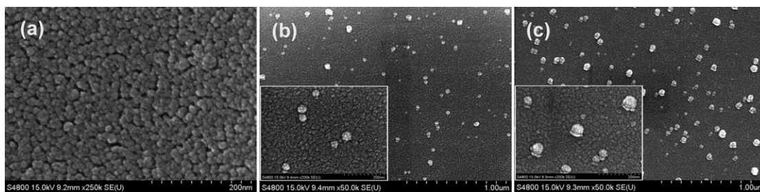
Fig. 1 SEM images of \text{TiO}_2 thin films. (a) \text{TiO}_2 films; (b) 0.25% Ag-loaded \text{TiO}_2 films; (c) 1.0% Ag-loaded \text{TiO}_2 films.
