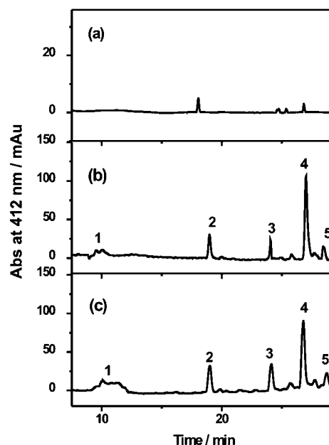
Fig. 3 Typical chromatograms without reduction (a), and with TBP (b) and UV-Ag/ \text{TiO}_2 -HCOOH (c). The identified peaks by HPLC-ESI-MS were GSH (1), \text{PC}_2 (2), \text{PC}_3 (3), \text{PC}_4 (4), \text{PC}_5 (5) (Fig. S5 \dagger ). Mobile phase A, 0.02% TFA- \text{H}_2\text{O} ; mobile phase B, 0.02% TFA-ACN; elution program: 0–25 min, B 2–25%; 25–30min, B 25%; flow rate, 0.15 \text{mL min}^{-1} ; derivatization conditions: 1.8 \text{mmol L}^{-1} DTNB, flow rate 0.05 \text{mL min}^{-1} ; detection wavelength, 412 nm.
