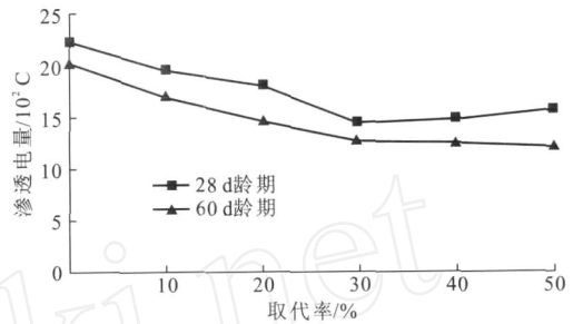
图 1 Ⅱ级粉煤灰对混凝土抗氯离子渗透性的影响 Fig. 1 Influences of II Fly Ash on Resistance Against Chloride Ion Penetration of Concrete
