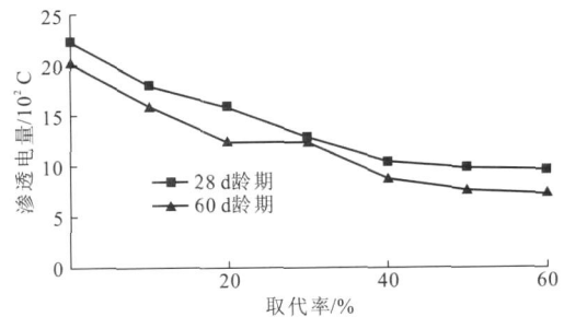
图 2 矿粉对混凝土抗氯离子渗透性的影响 Fig. 2 Influences of Slag Powder on Resistance Against Chloride Ion Penetration of Concrete
