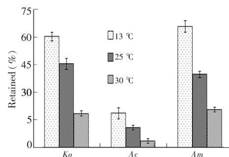
图4 不同温度条件下,消减过程结束时(180 h)3种红树叶片表面菲的百分残留量 Fig. 4 Percentage of Phen retained on three mangrove leaf surface after 180 h depuration under different temperatures
